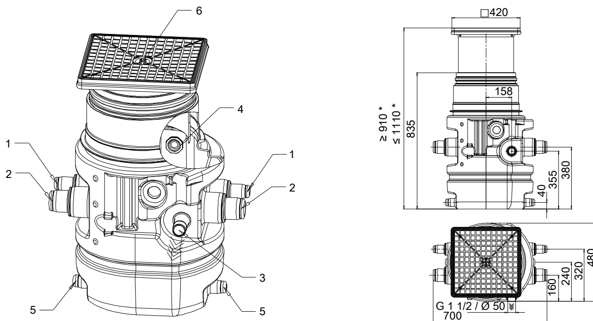
Fig. 1: Connections and dimensions of a single-pump lifting unit
