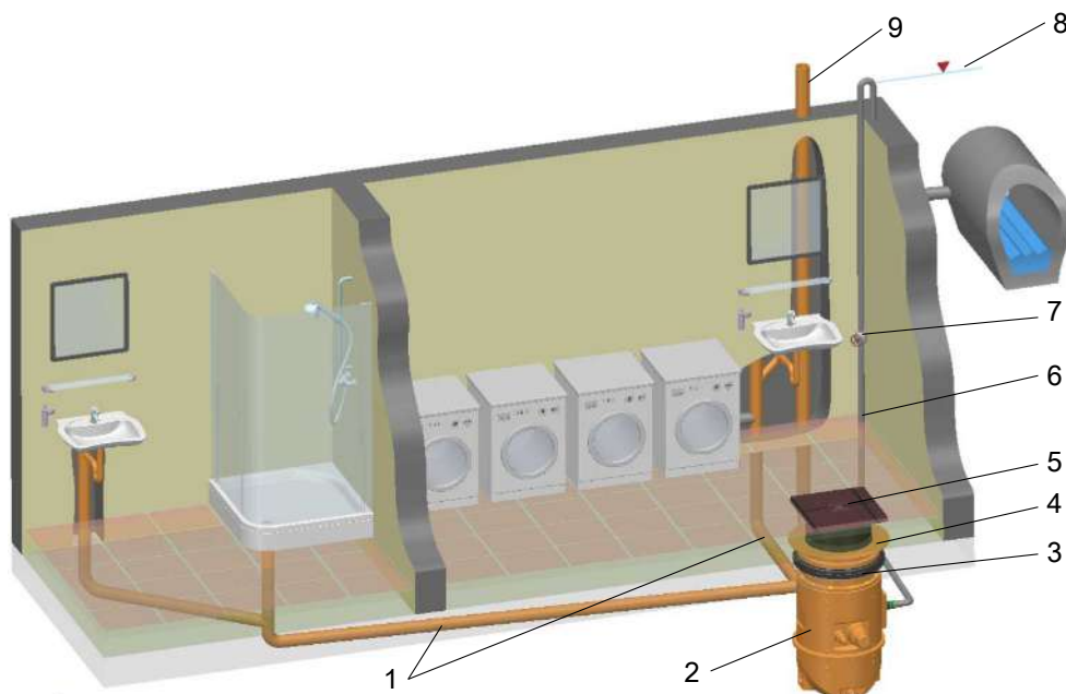
Fig. 6: Installation example
