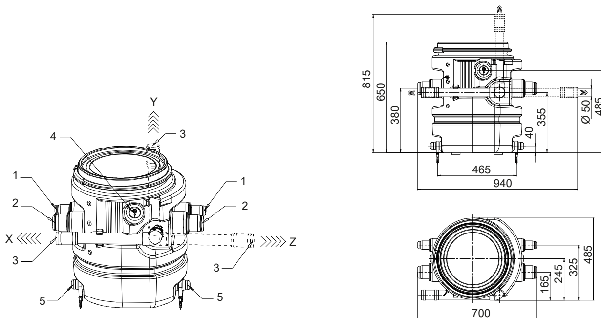
Fig. 3: Connections and dimensions of a single-pump lifting unit
