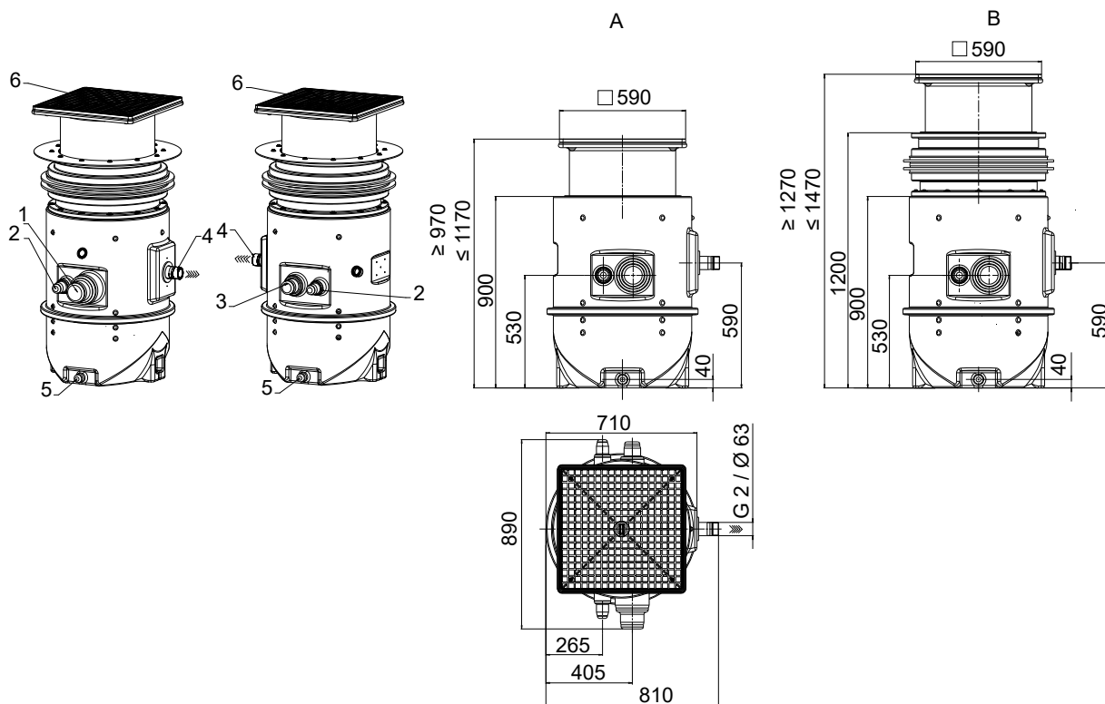
Fig. 2: Connections and dimensions of a dual-pump lifting unit
