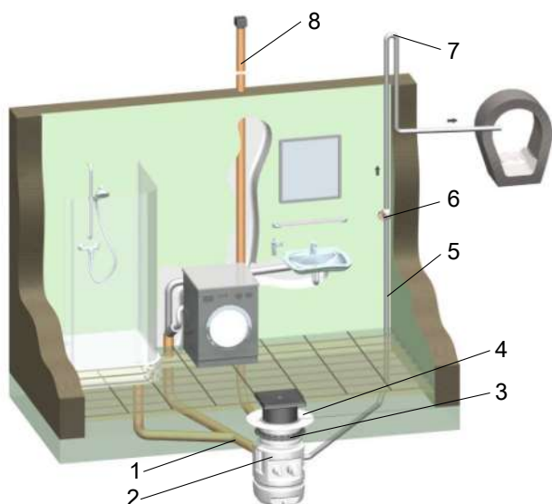
Fig. 5: Installation example
