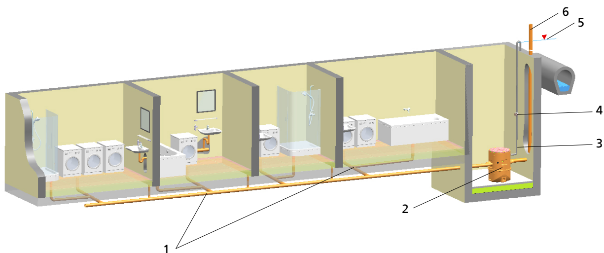
Fig. 8: Installation example
