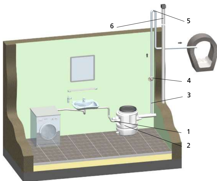
Fig. 7: Installation example
